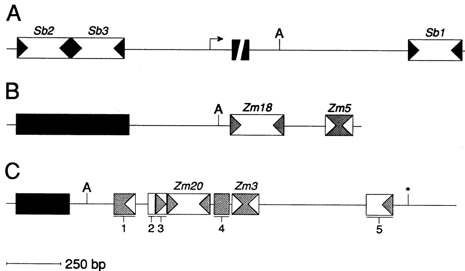
Fig. 2. Complete and partial Tourist elements in the flanking regions of the sorghum hydroxyproline-rich glycoprotein gene (A) and maize oleosin (B) and Adh1-C m genes (C). Tourist element locations are shown relative to coding regions (solid box), transcription start sites (bent arrow), and polyadenylation signals (A). Element subfamilies are indicated by shaded boxes with open inverted arrows ( Tourist A ), open boxes with dark shaded inverted arrows ( Tourist B ), and open boxes with light shaded inverted arrows ( Tourist D ). Inverted arrows indicate TIRs and are not drawn to scale. Boxes corresponding to partial elements (boxes 1–5) in the 3' flanking region of the maize Adh1-C m allele are shaded to indicate their Tourist subfamily affiliation. The insertion site of Tourist-Zm8 in the maize Adh1-1S allele is marked by an asterisk.
